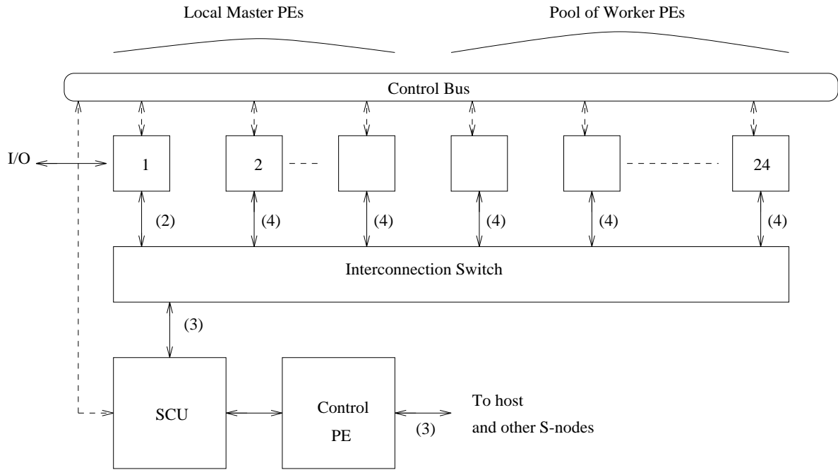
Figure 2: Parsys SuperNode Architecture
