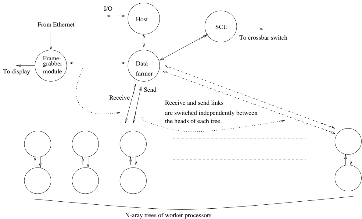
Figure 3: Set-up for Dynamically-Switched Network with Local Communication
