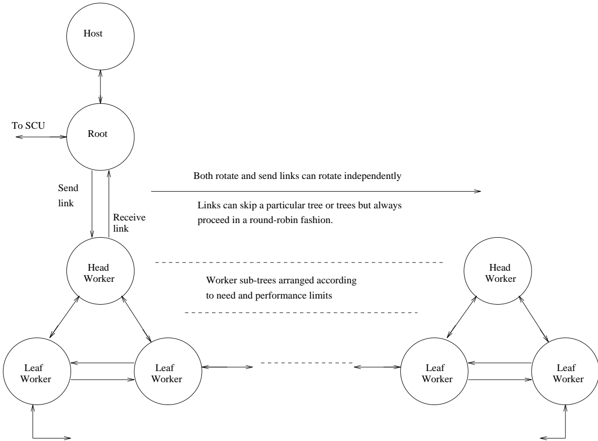
Figure 4: Set-up for Dynamically-Switched Network with Global Communication
